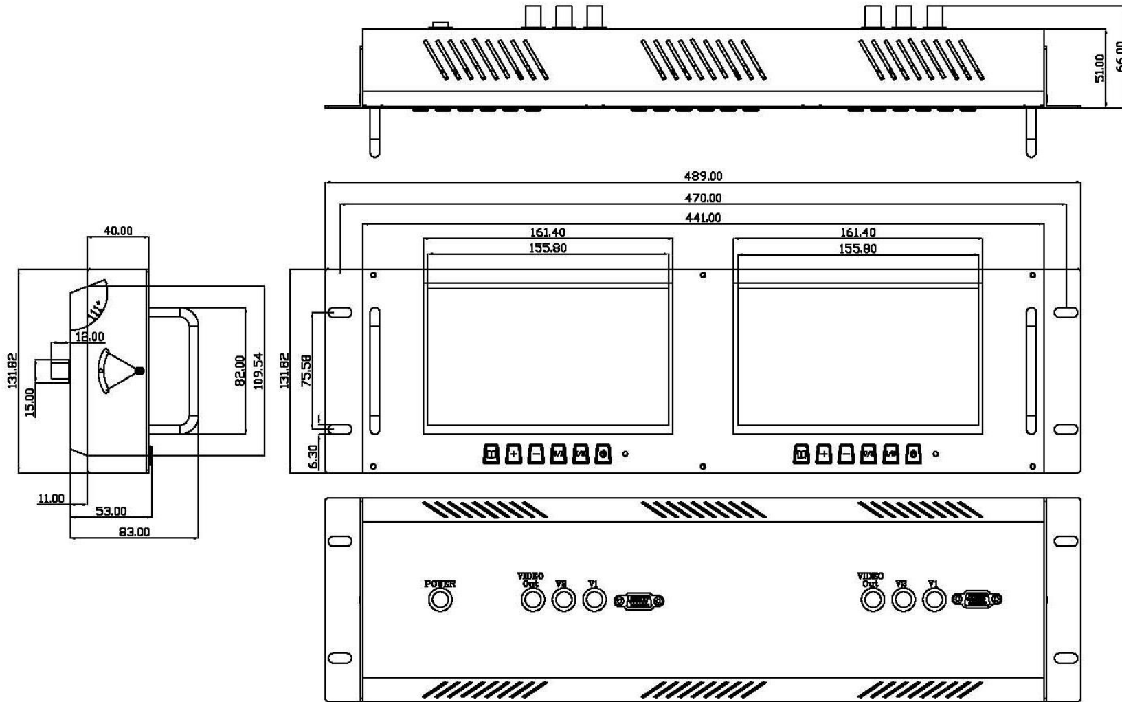
Line Drawing for: Model No. LRM7531 All sizes are in mm Drawing not to scale.
