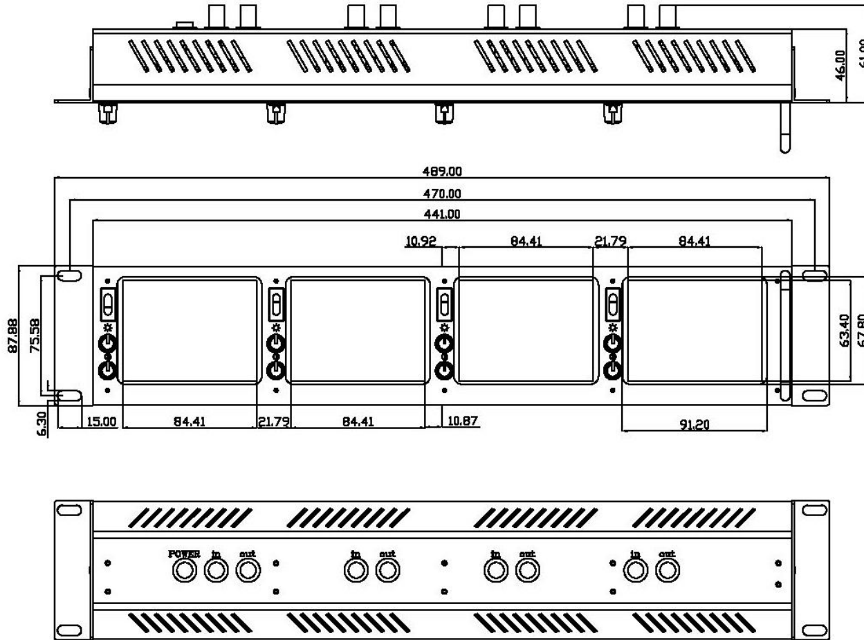
Line Drawing for: Model No. LRM4521 All sizes are in mm Drawing not to scale.
