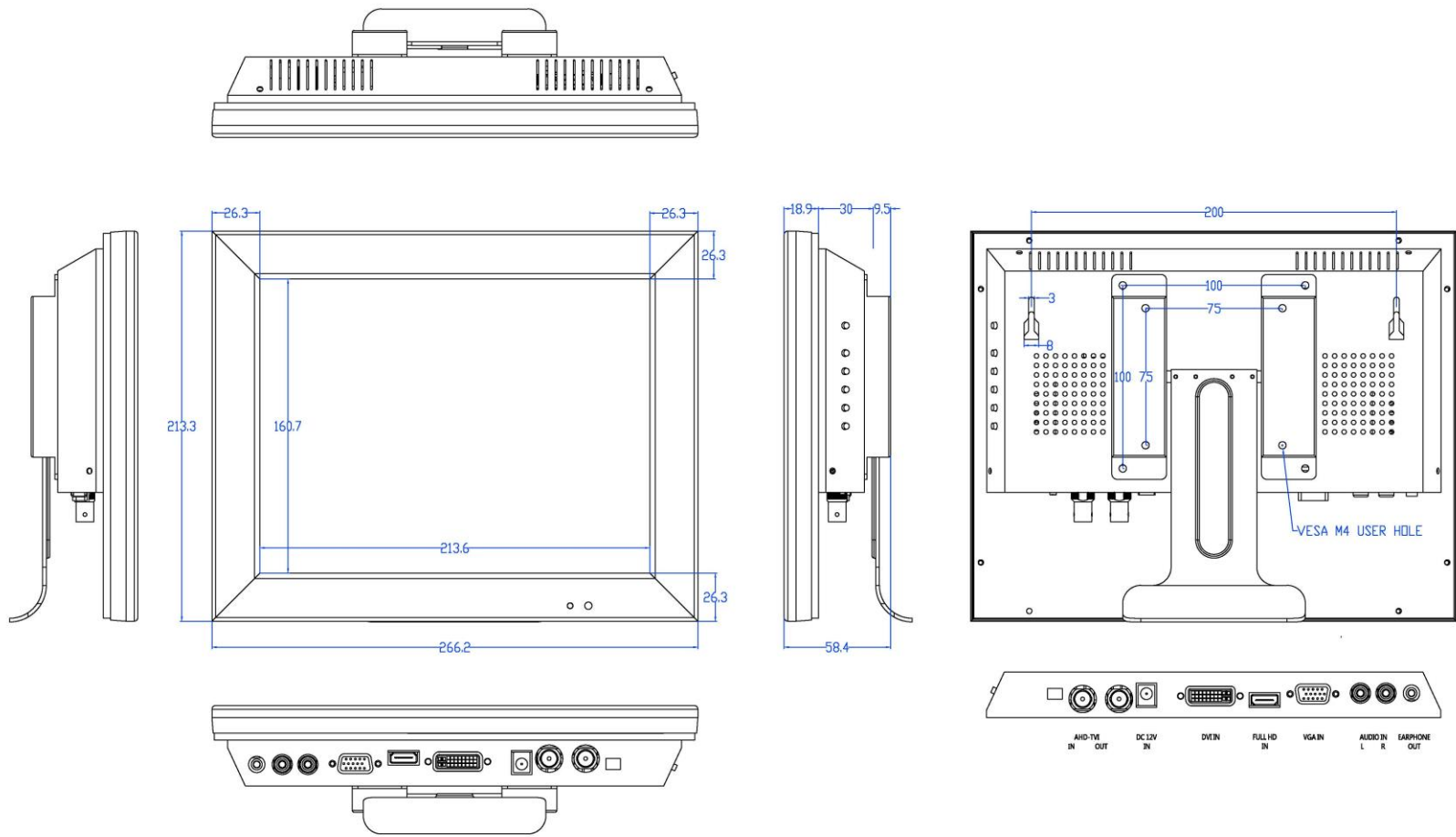
Line Drawing for: Model No. L104AT All sizes are in mm Drawing not to scale.
