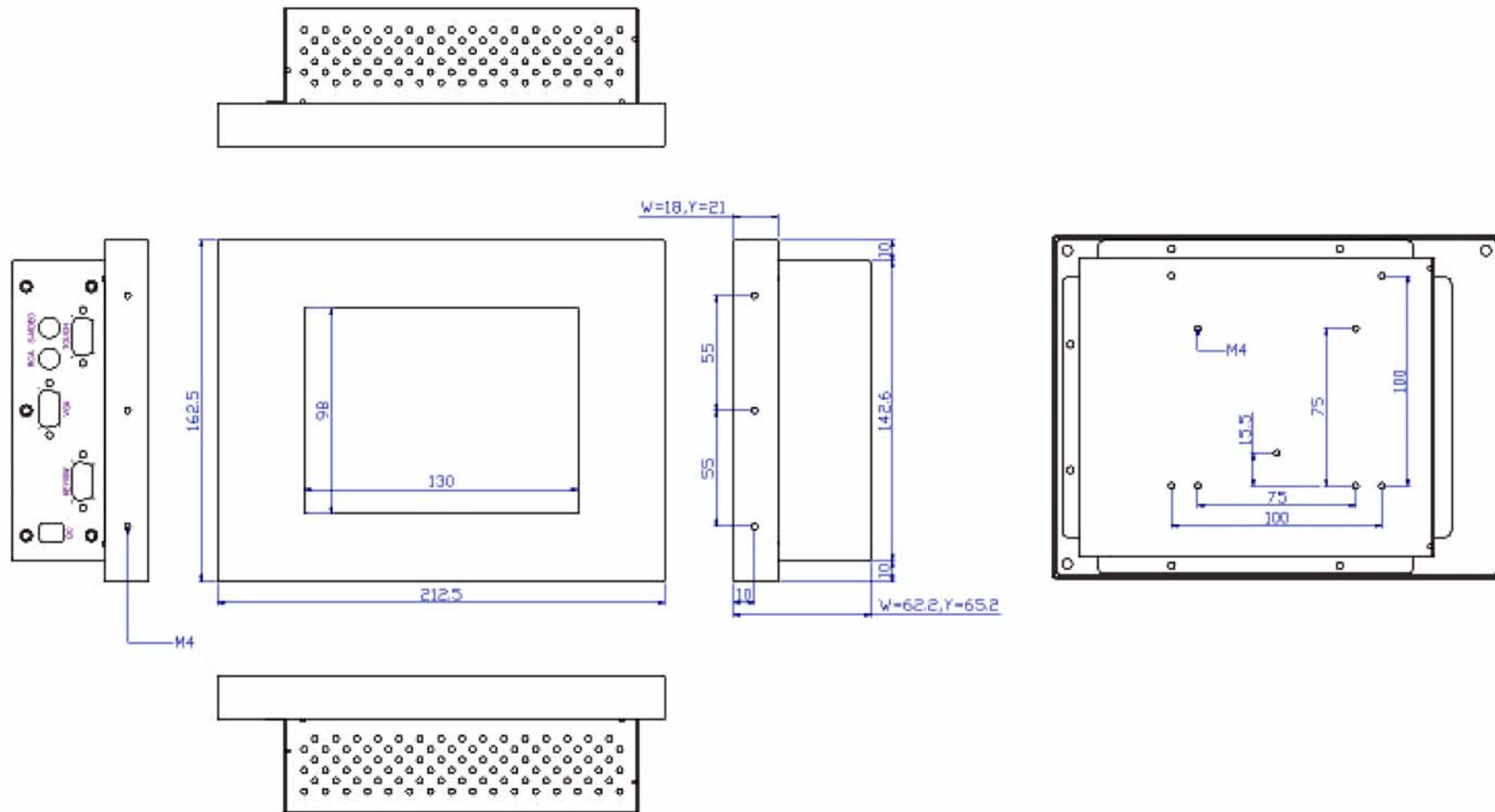
Line Drawing for: Model No. 64W12P All sizes are in mm
