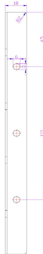
Line Drawing for: Model No. 10W12U All sizes are in mm
