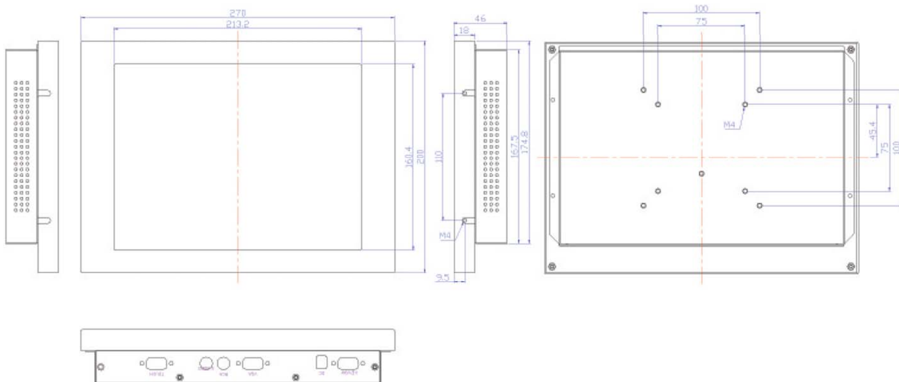
Line Drawing for: Model No. 10W12U All sizes are in mm
