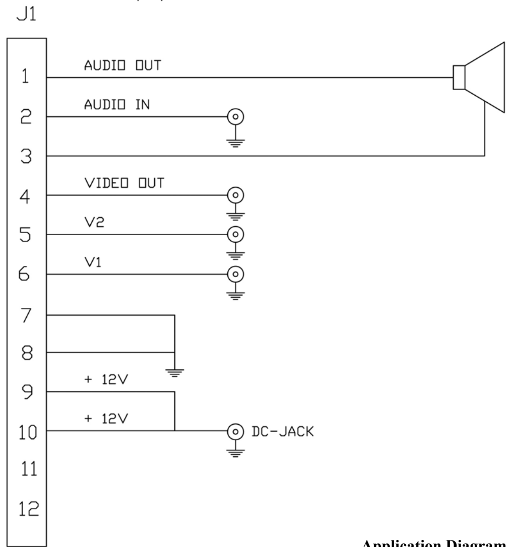
Application Diagram for: Model No. LCD7323mod IO All sizes are in mm
